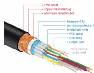
Triple shielding for lossless signal transfer
