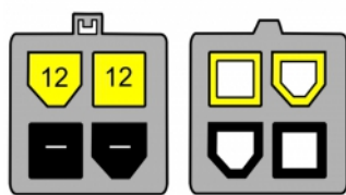
Stecker male
